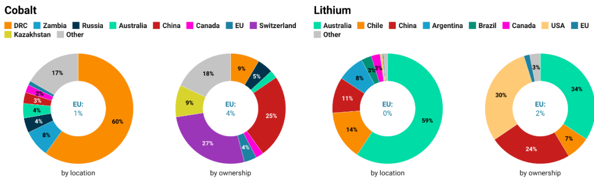
Figure 15. Cobalt and lithium mine capacity by location and owner company headquarter in 2020
