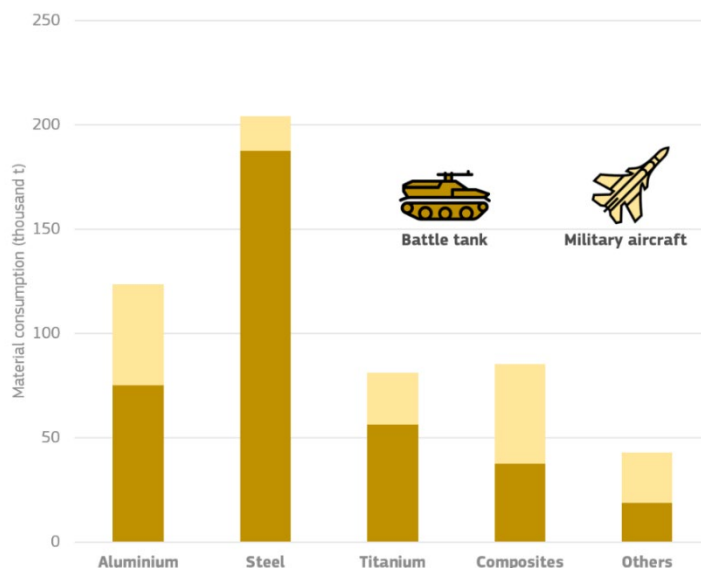
Figure 107. Demand for structural materials in NATO fleets of aircrafts and battle tanks as of 2022 74 .
