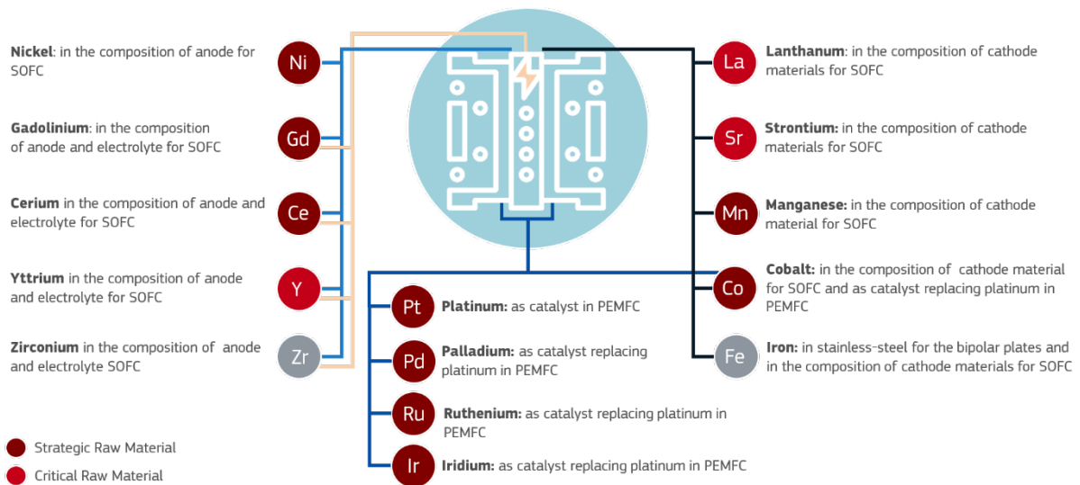
Figure 16. Selection of raw materials used in fuel cells and their function
