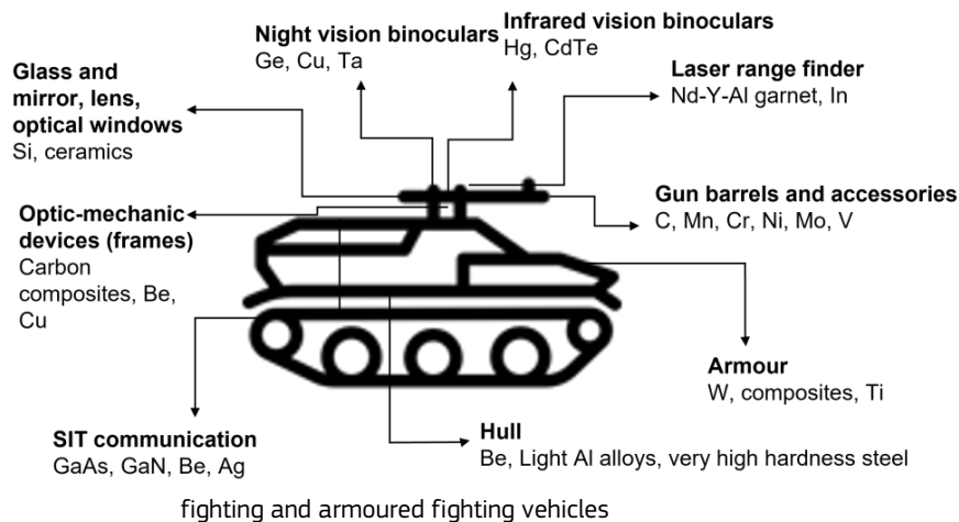
Figure 108. Components and raw materials used in a main battle tank (e.g. Leclerc), but also representative of infantry-
