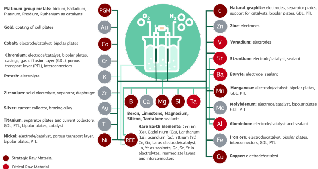
Figure 21. Selection of raw materials used in electrolysers and their function
