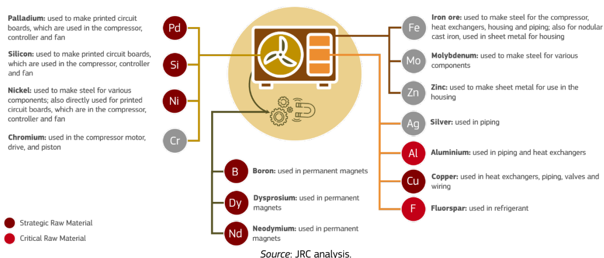
Figure 47. Selection of raw materials used in heat pumps and their function
