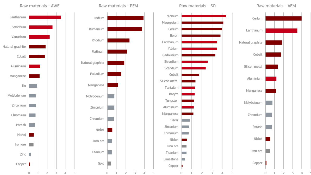
Figure 23. Detailed Supply Risk of selected raw materials in the electrolyzers supply chain
