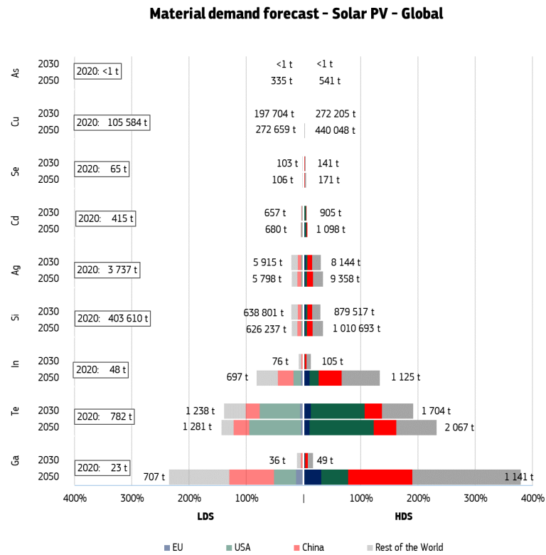
Figure 45. Material demand forecast for solar PV: global (top) and focus on the EU (bottom)
