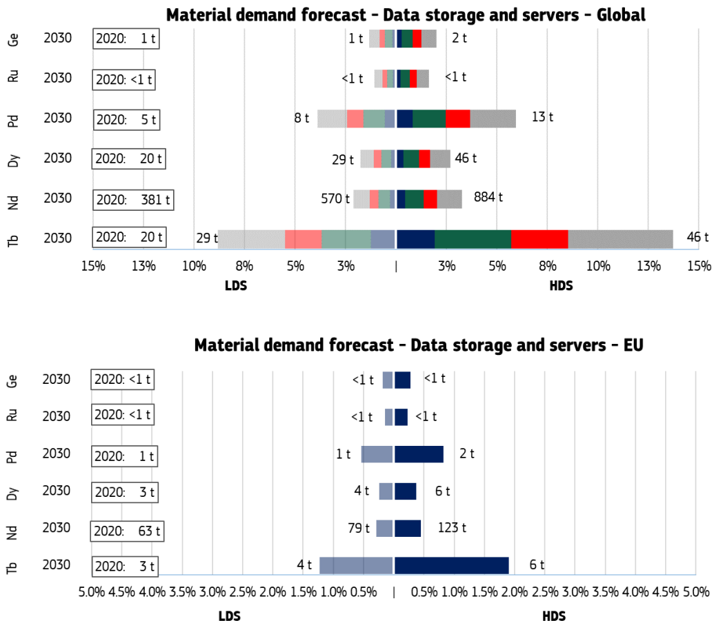
Figure 63. Material demand forecast for data storage and servers: global (top) and focus on the EU (bottom)
