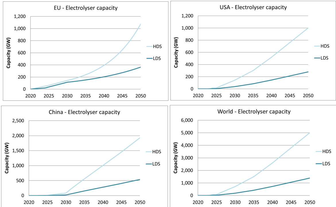
Figure 26. Electrolyser capacity in the EU, US, China, and globally in the two explored scenarios
