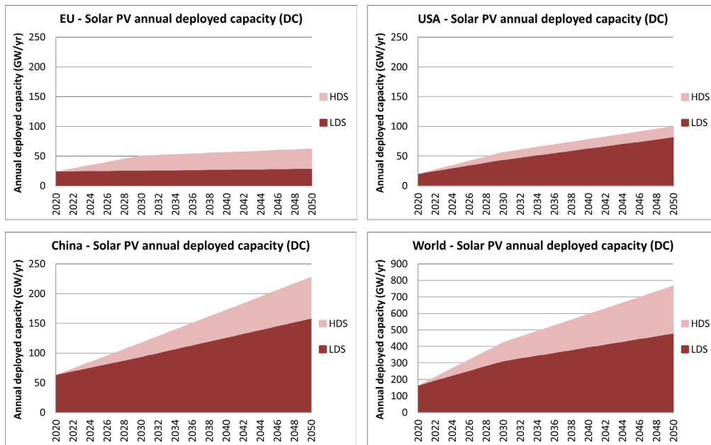
Figure 44. Solar PV annual deployed capacity in the EU, US, China, and globally in the two explored scenarios
