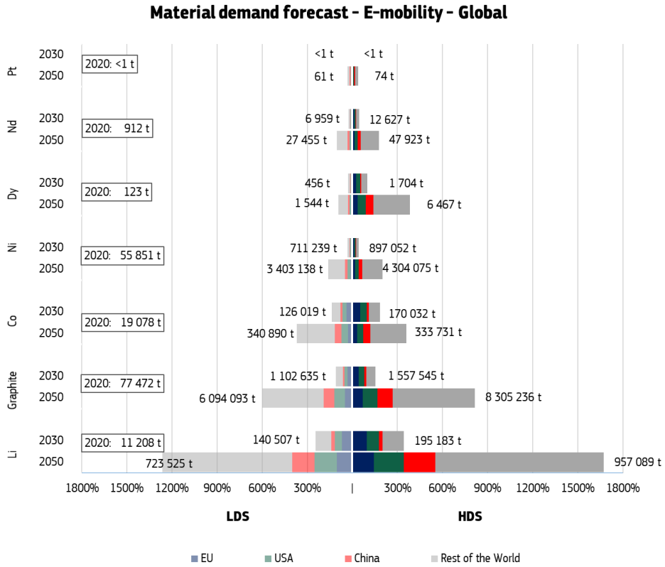
Figure 93. Material demand forecast for the e-mobility sector: global (top) and focus on the EU (bottom)
