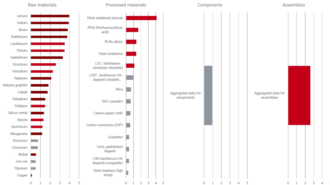
Figure 18. Detailed Supply Risk of all elements in the fuel cell supply chain
