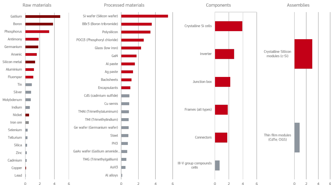
Figure 42. Detailed Supply Risk of selected elements in the Solar PV supply chain
