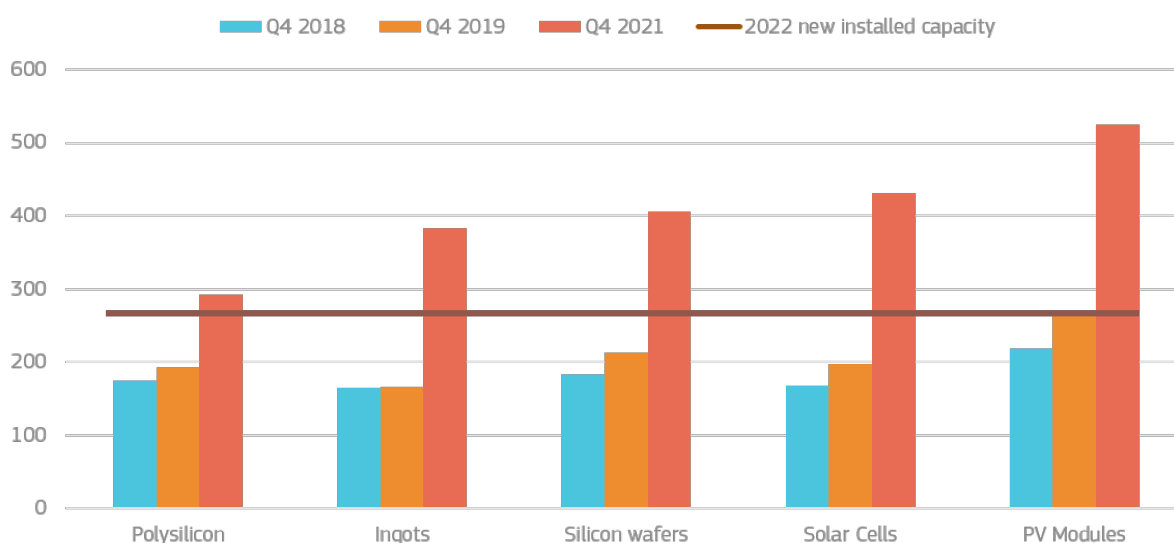
Figure 46. Global year-end silicon PV supply chain manufacturing capacity versus 2022 global new installation (in GW/year)
