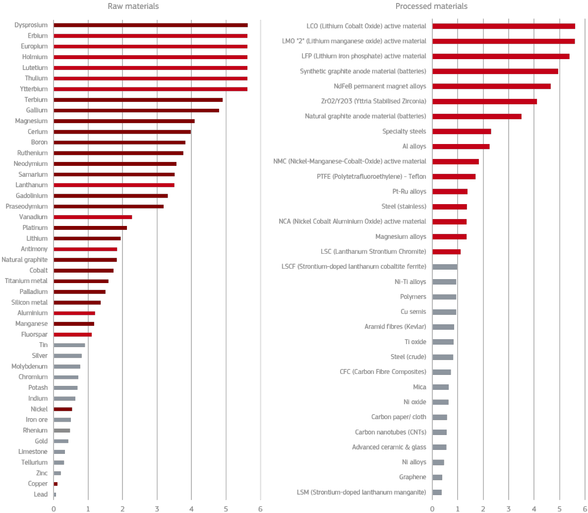
Figure 74. Detailed Supply Risk of selected elements in the robotics supply chain
