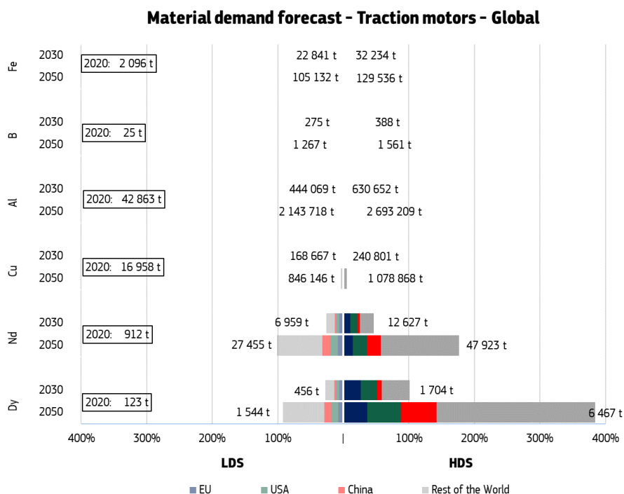
Figure 39. Material demand forecast for traction motors: global (this page) and focus on the EU (next page)
