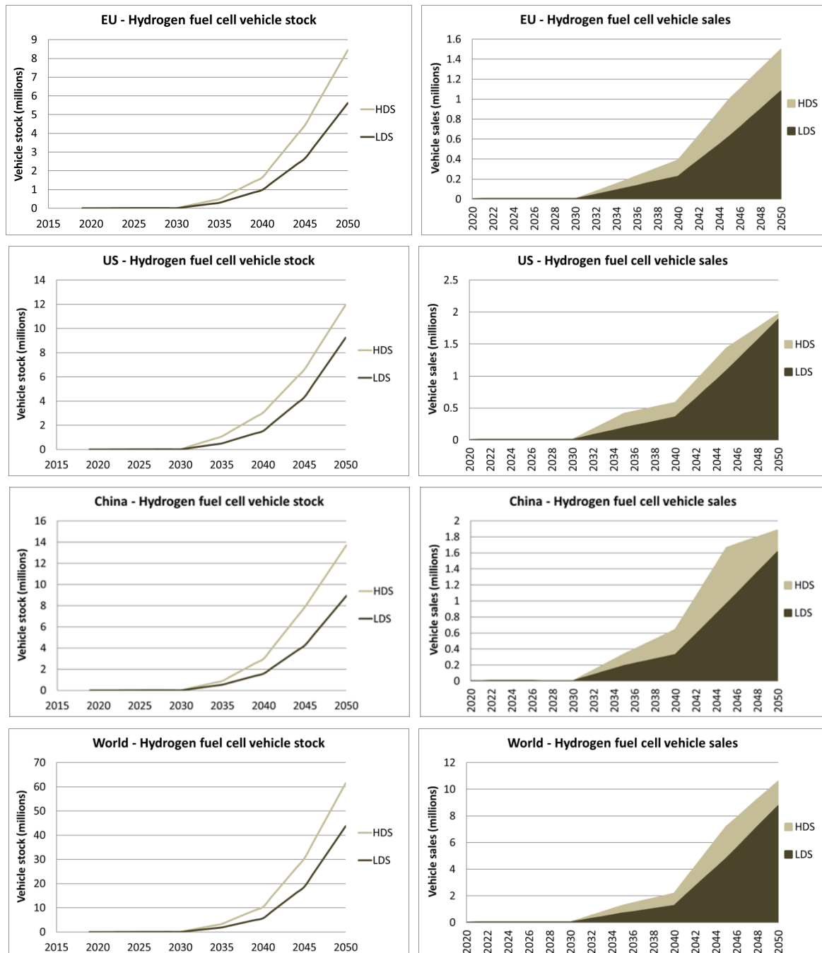
Figure 19. Fleet and annual sales of fuel cell vehicles in the EU, US, China, and globally in the two explored scenarios
