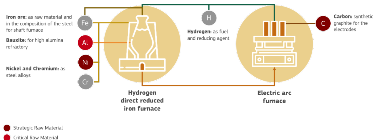
Figure 52. Selection of raw materials used in H 2 -DRI ironmaking and EAF steelmaking and their function
