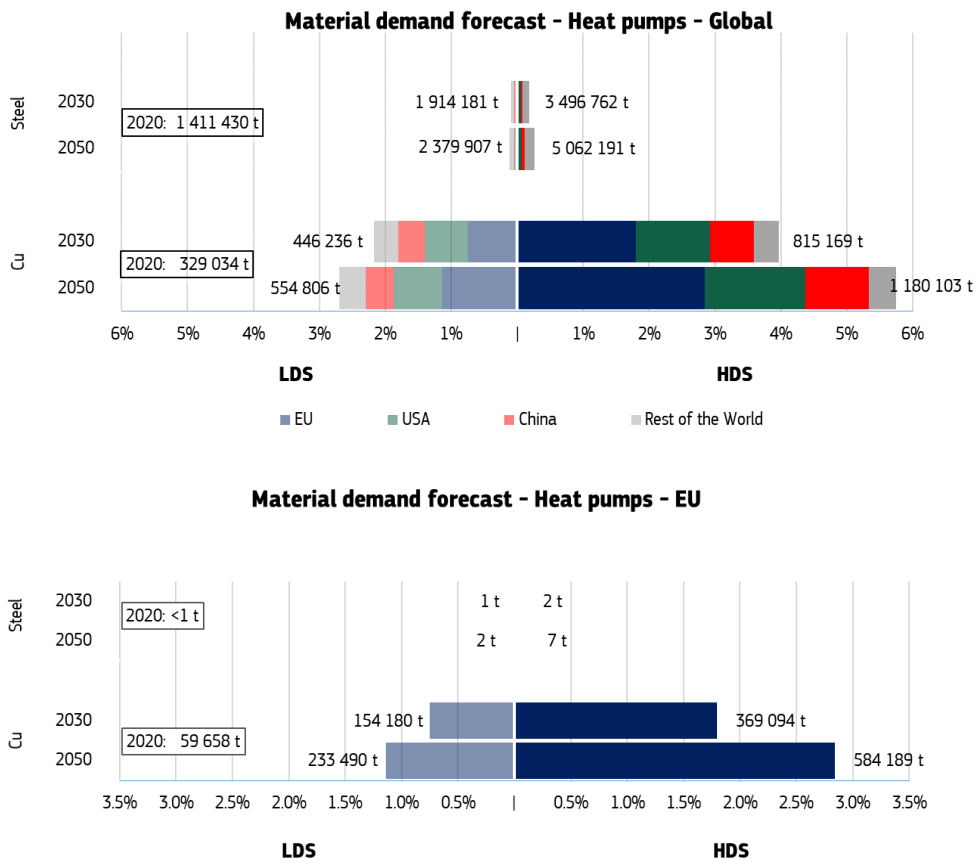
Figure 51. Material demand forecast for heat pumps: global (top) and focus on the EU (bottom)
