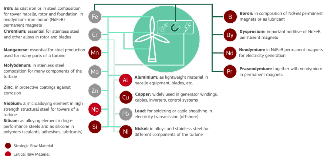
Figure 30. Selection of raw materials used in wind turbines and their function
