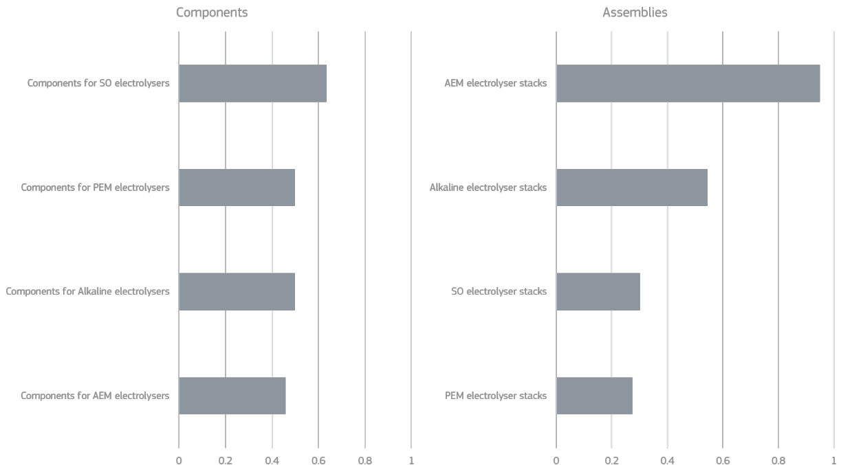
Figure 25. Detailed Supply Risk of components and stacks in the electrolyzers supply chain
