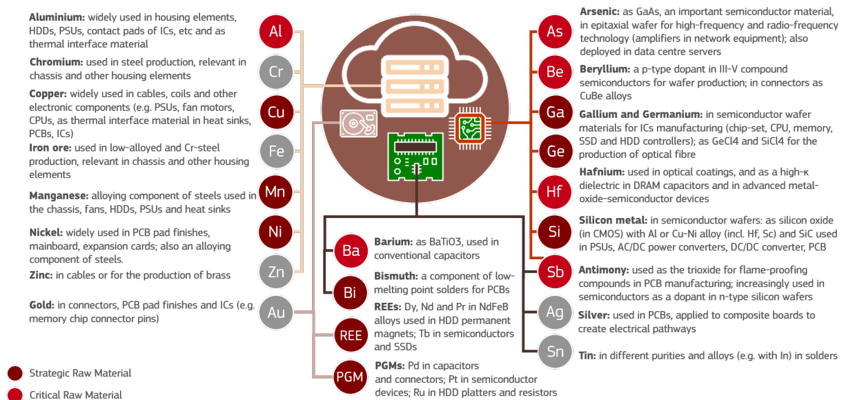
Figure 59. Selection of raw materials used in data storage and servers, and their function.
