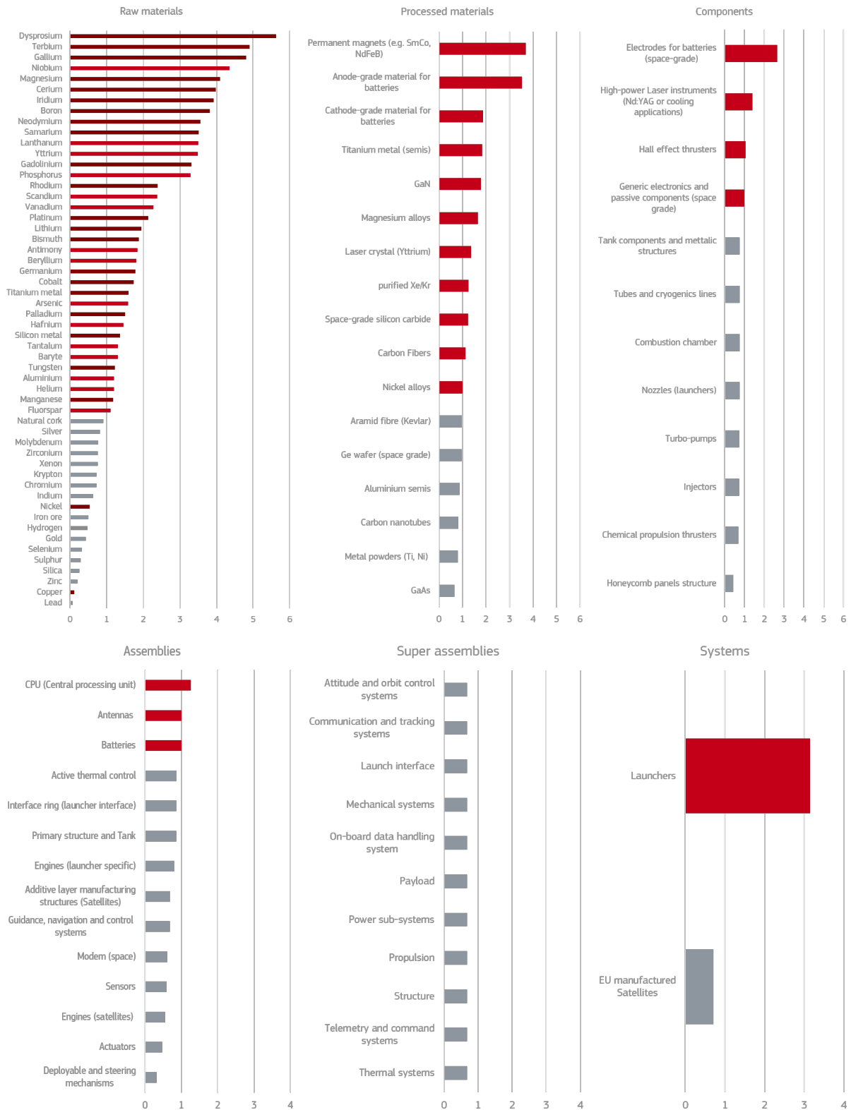
Figure 80. Detailed Supply Risk of selected elements in the space launchers and satellites supply chain
