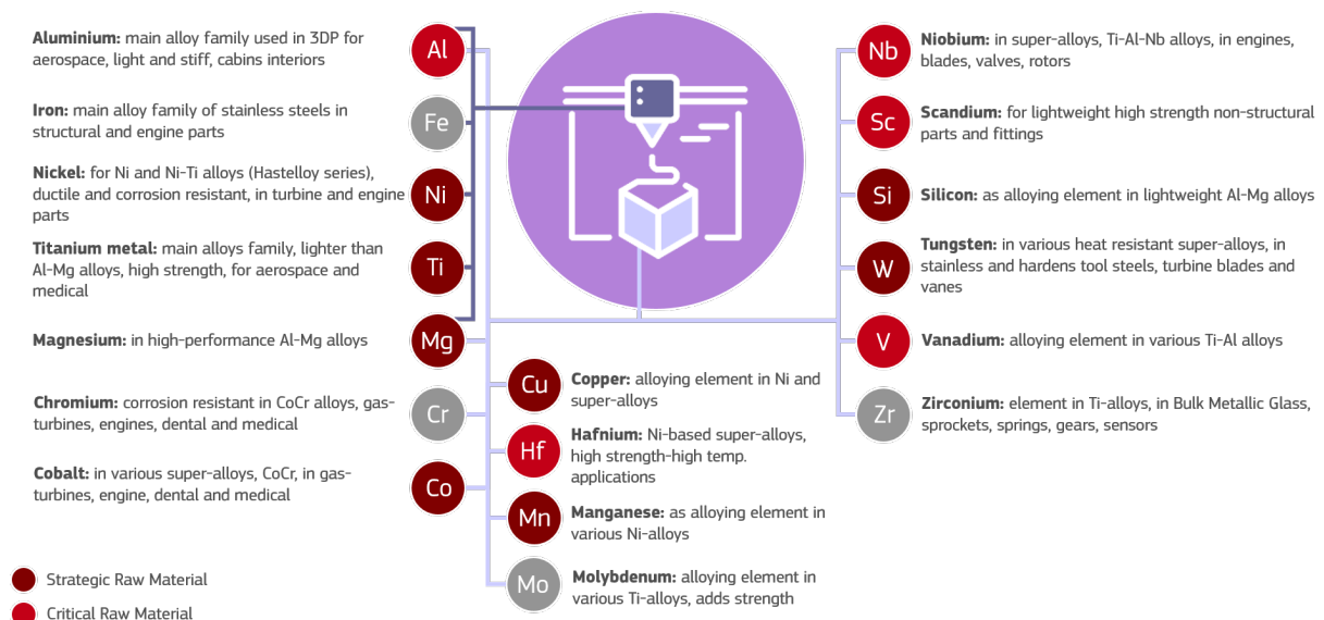
Figure 69. Selection of raw materials used in additive manufacturing (3D printing) and their function
