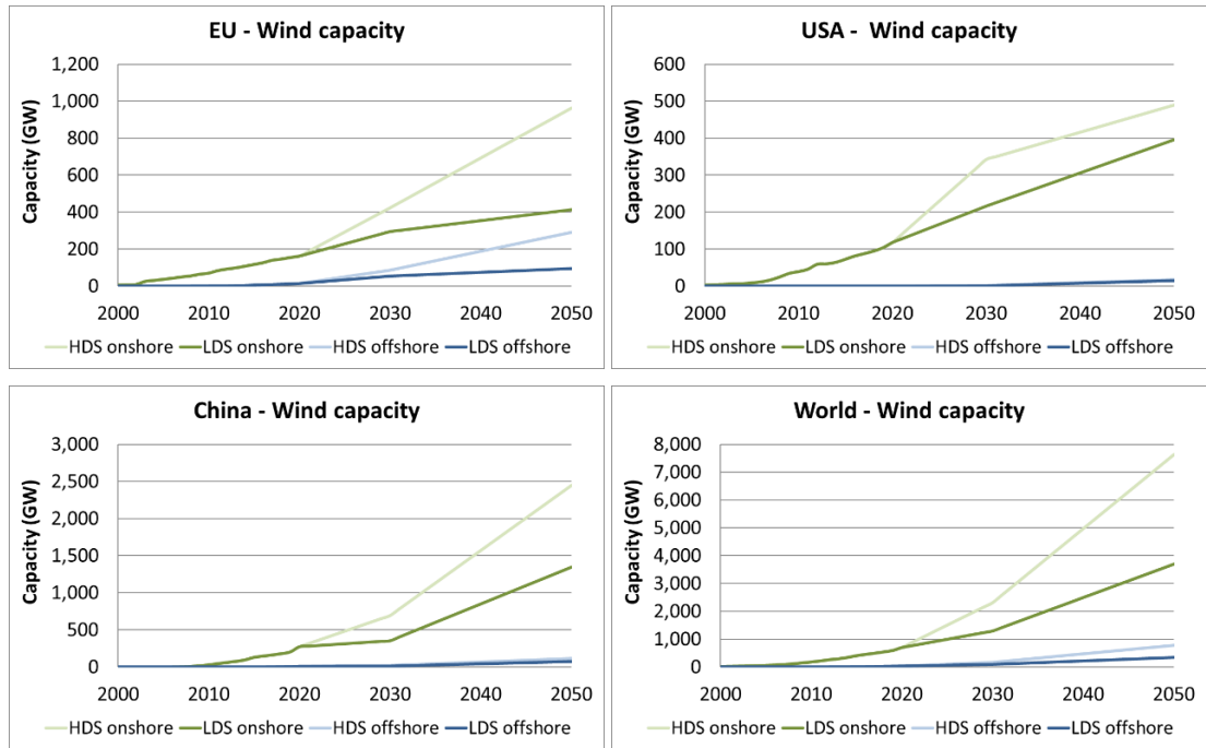
Figure 33. Onshore and offshore wind capacity in the EU, US, China, and globally in the two explored scenarios
