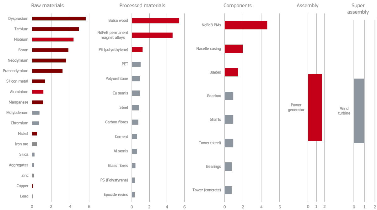
Figure 32. Detailed Supply Risk of all elements in the wind turbine supply chain
