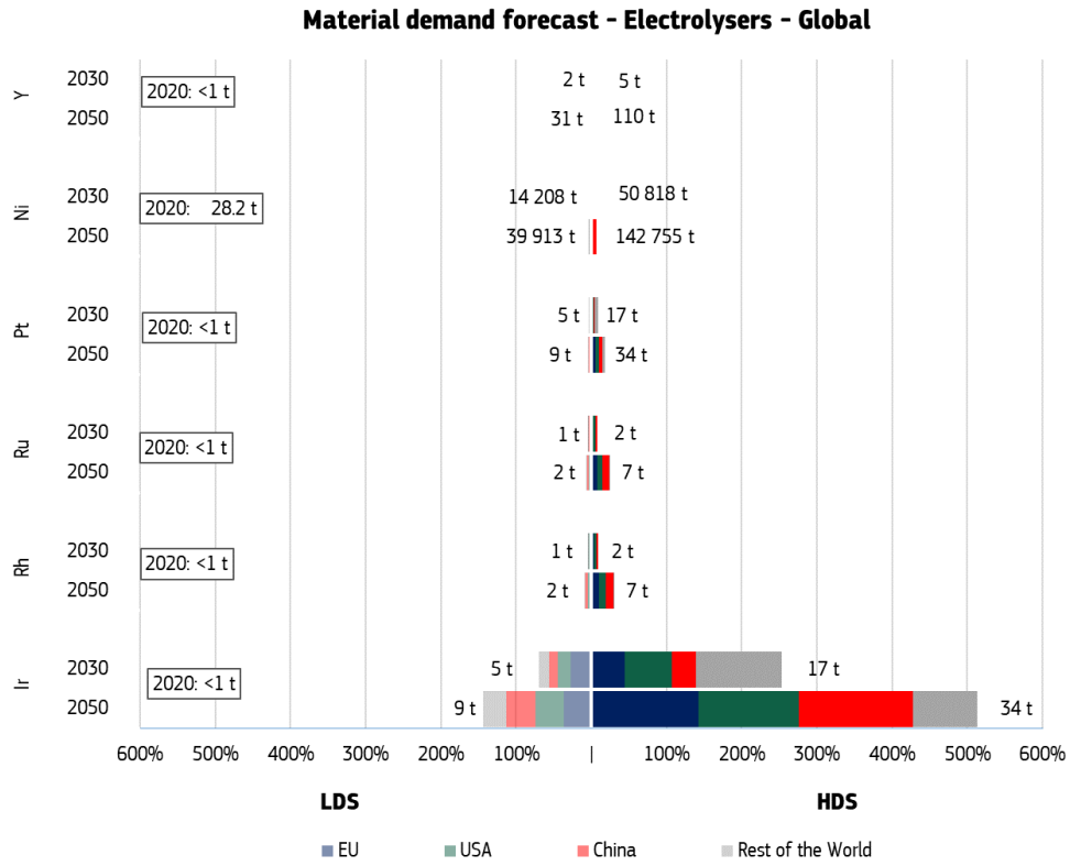
Figure 29 Material demand forecast for electrolyzers: global (top) and focus on the EU (bottom)
