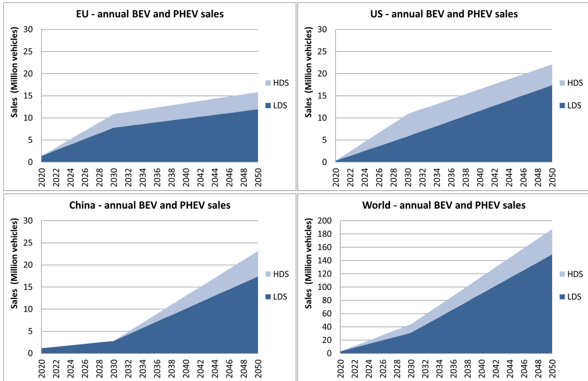
Figure 10. Annual sales of battery (BEVs) and plug-in (PHEVs) electric vehicles in the EU, US, China, and globally in the two explored scenarios
