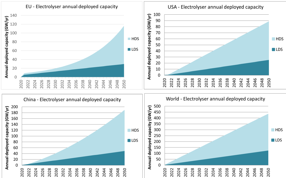
Figure 27. Electrolyser annual deployed capacity in the EU, US, China and globally in the two explored scenarios
