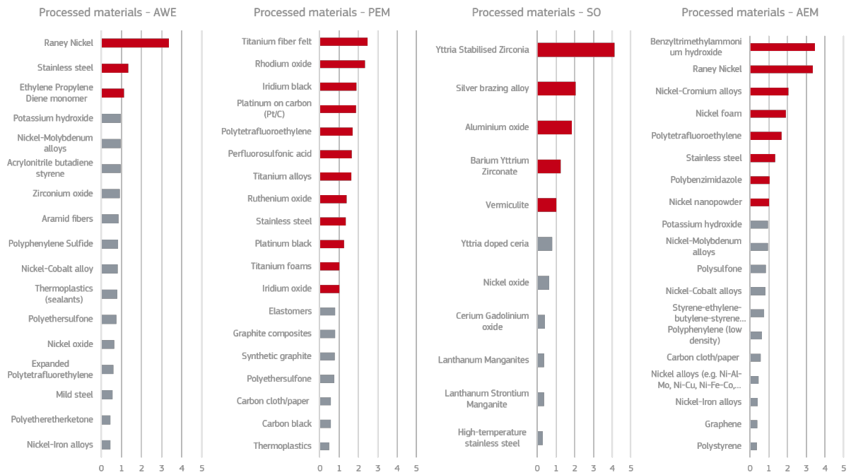
Figure 24. Detailed Supply Risk of selected processed materials in the electrolyzers supply chain
