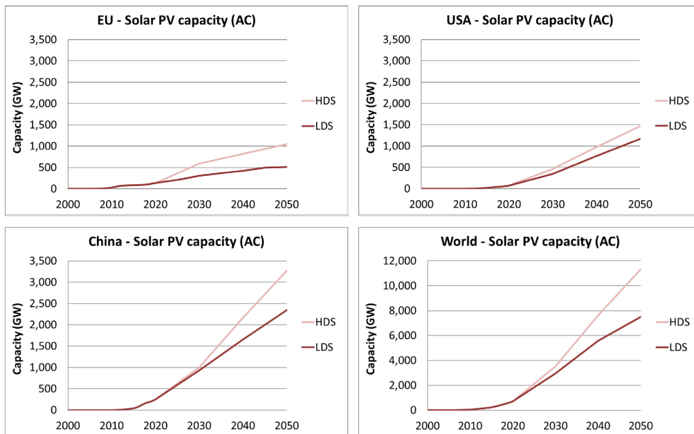
Figure 43. Solar PV capacity in the EU, US, China, and globally in the two explored scenarios
