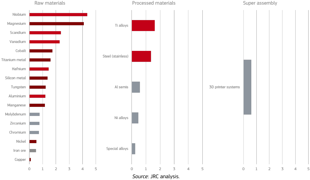
Figure 71. Detailed Supply Risk of selected elements in the data transmission networks supply chain
