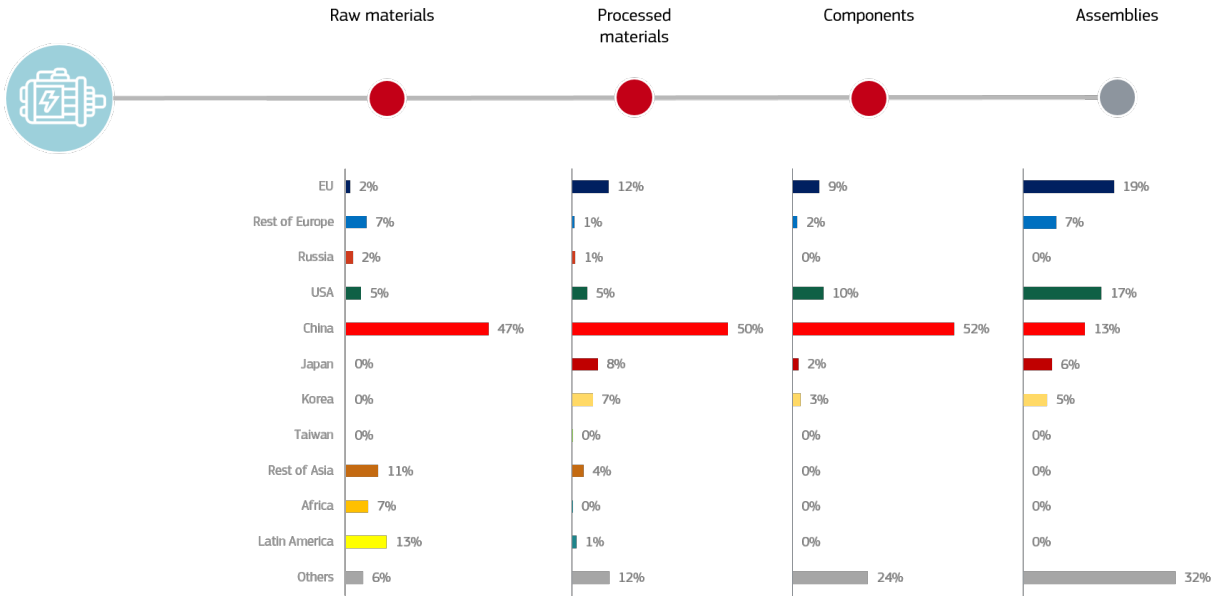
Figure 37. An overview of supply risks, bottlenecks, and key players along the supply chain of traction motors
