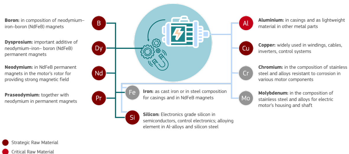
Figure 36. Selection of raw materials used in traction motors and their function
