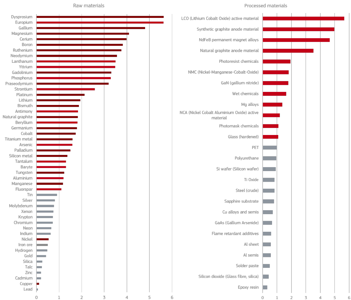
Figure 66. Detailed Supply Risk of selected elements in the smartphones, tablets and laptops supply chain
