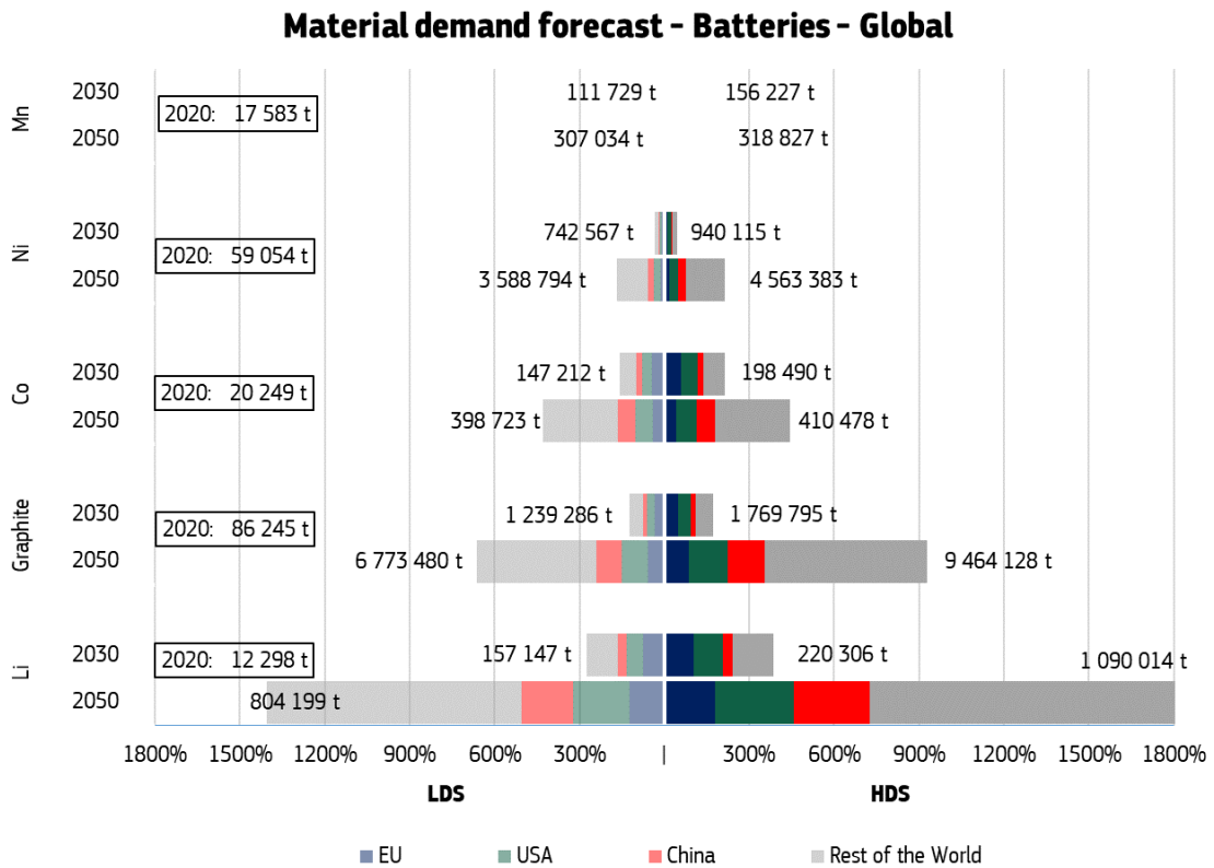
Figure 13. Material demand forecast for Li-ion batteries: global (top) and focus on the EU (next page)
