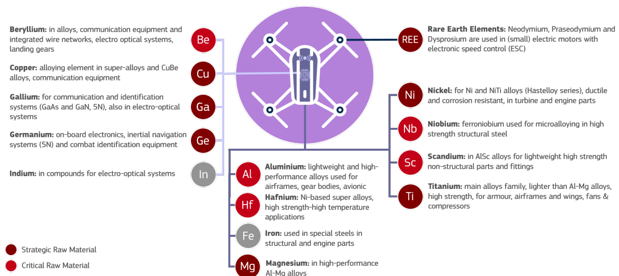
Figure 75. Selection of raw materials used in drones and their function
