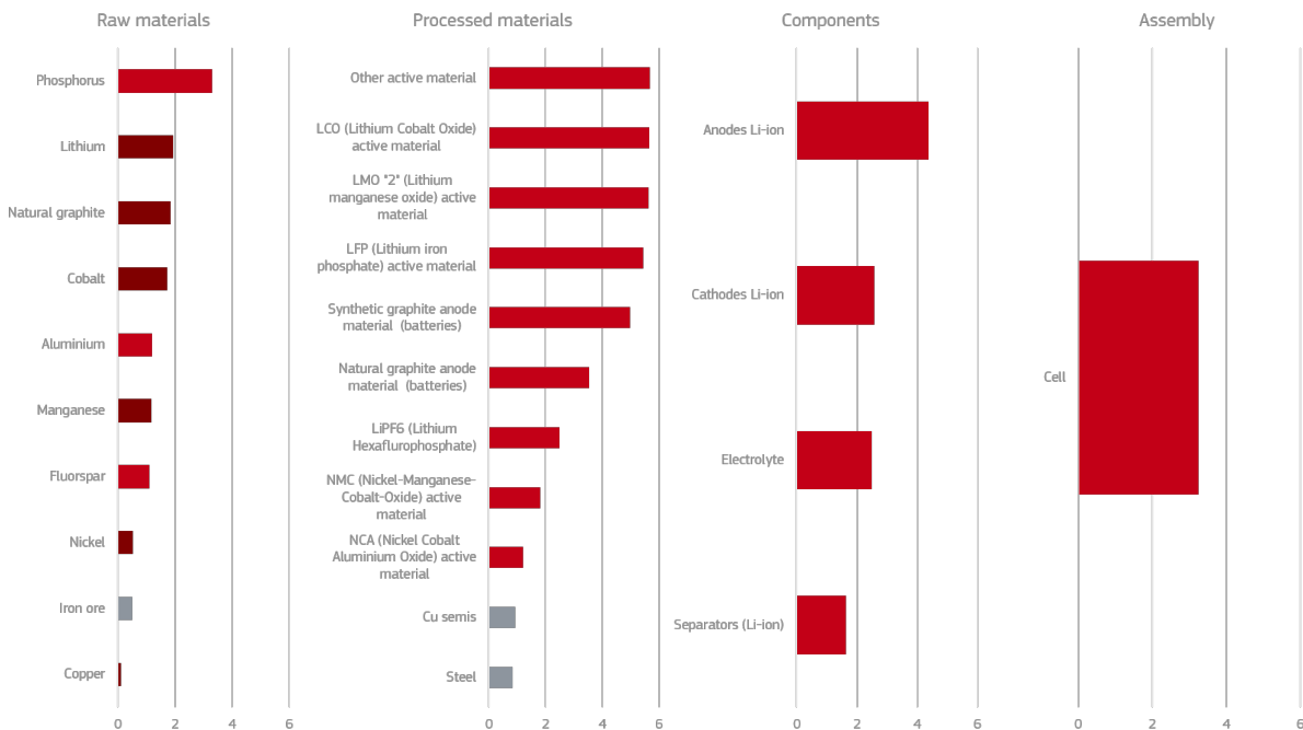
Figure 9. Detailed Supply Risk of all elements in the Li-ion battery supply chain
