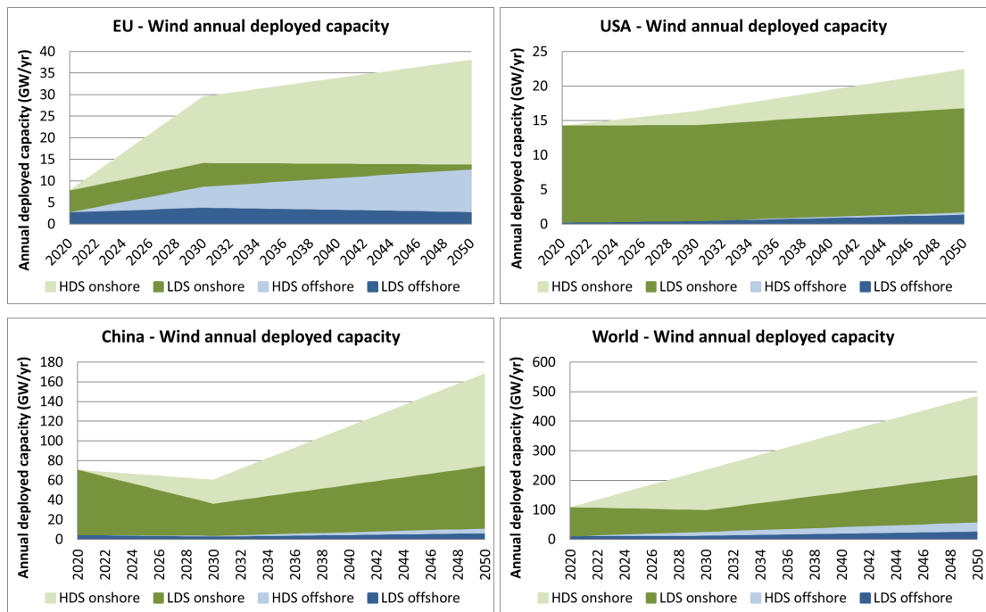
Figure 34. Onshore and offshore wind annual deployed capacity in the EU, US, China, and globally in the two explored scenarios
