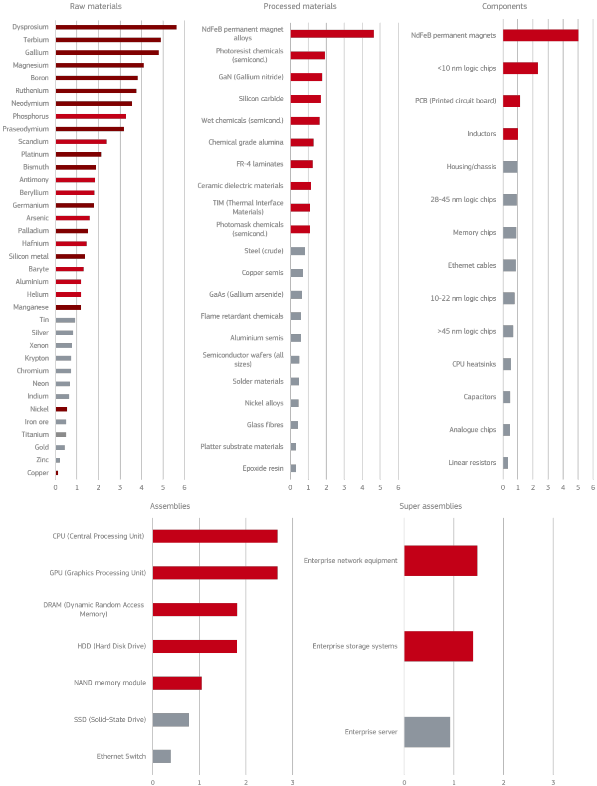
Figure 61. Supply bottlenecks along the value chain of data servers and storage.
