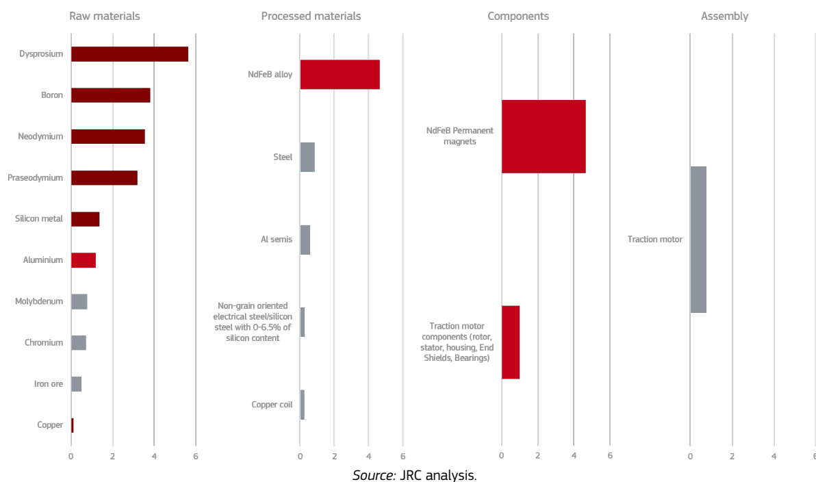
Figure 38. Detailed Supply Risk of all elements in the traction motors supply chain
