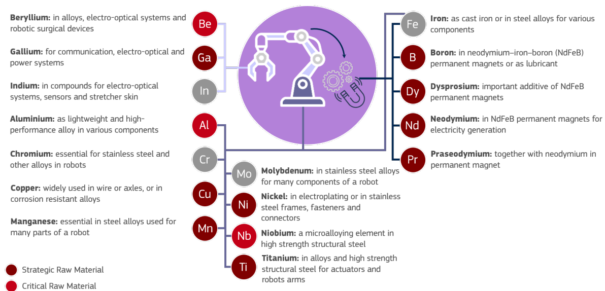
Figure 72. Selection of raw materials used in robotics and their function
