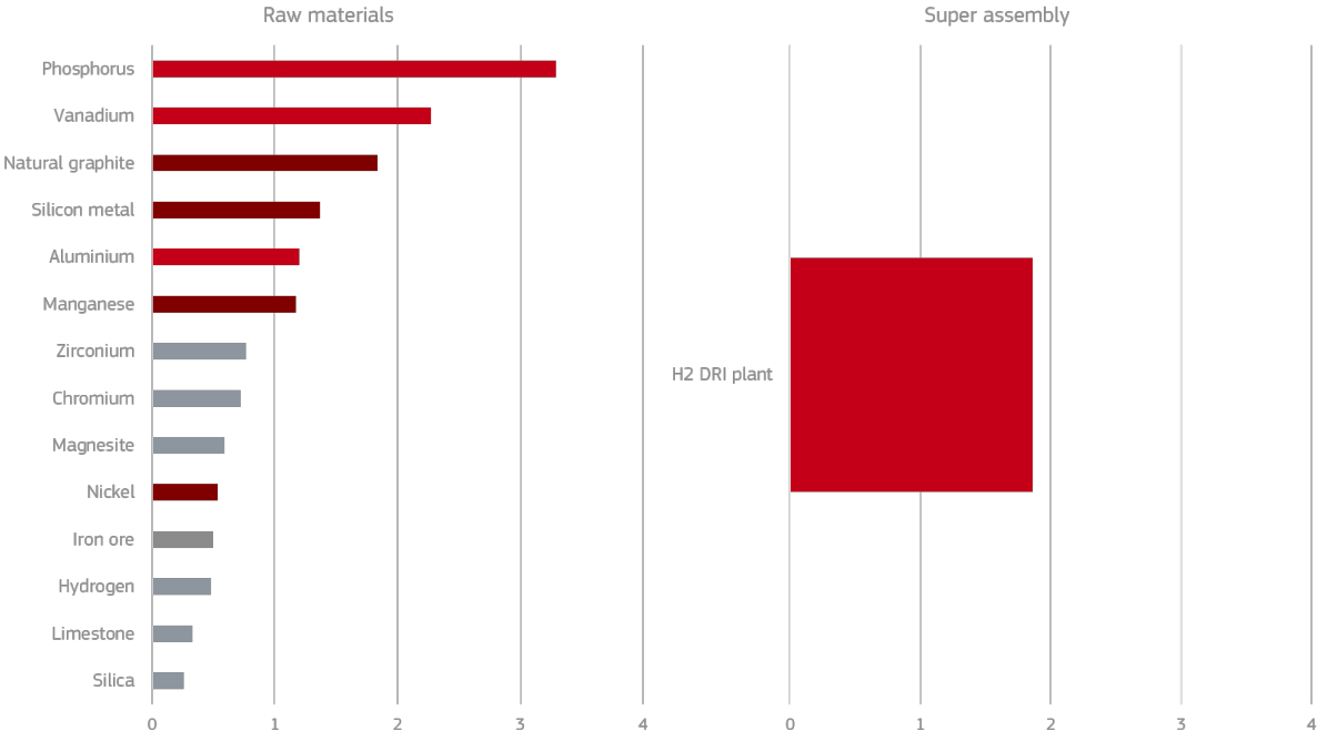
Figure 54. Detailed Supply Risk of selected elements in the H2-DRI ironmaking supply chain
